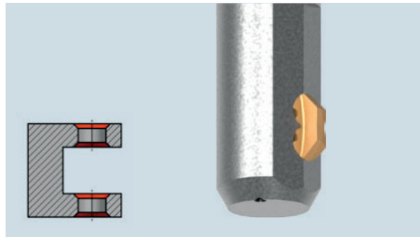
Chamfering front and back
