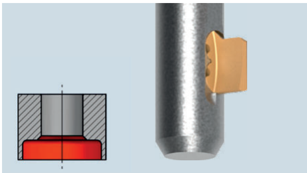
Formsinking backward
