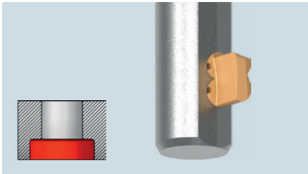
Back Spotfacing
