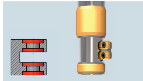
Counterboring forward and backward by insert holder with inserts
